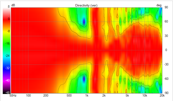
Vertical Polar Plot
