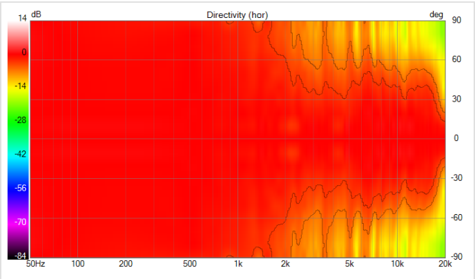
Horizontal Polar Plot
